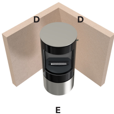
Corner installation
